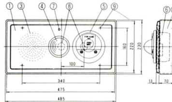
Surface Mounting Type SR-01M4L-47SD (P-1 Type) SR-02M4L-47SD (P-2 Type)
