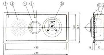
Recessed Mounting Type SU-01M4L-47SD (P-1 Type) SU-02M4L-47SD (P-2 Type)
